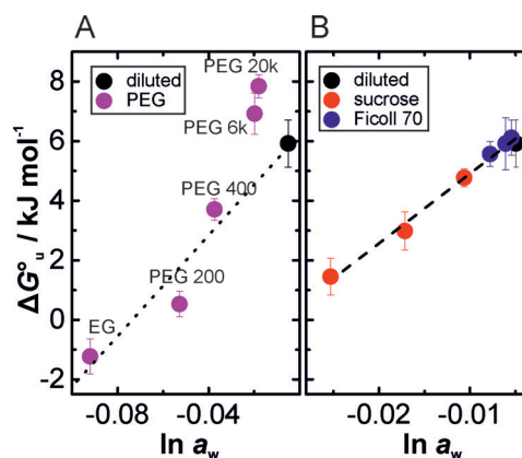
Figure 2. Im-4U RNA folding stability in different crowded solutions in vitro. The free energy for unfolding at 37^\circ\text{C} , \Delta G^\circ_u , is plotted against the activity of water, \ln a_w . The DPBS buffer is used as diluted reference buffer. A) Size-dependent effect of PEG ( 300 \text{ g L}^{-1} ) on the RNA folding stability. The dotted line indicates the dependence of the folding stability on \ln a_w for PEG < 6 kDa. B) Concentration-dependent effect of sucrose and Ficoll 70 (100, 200, and 300 \text{ g L}^{-1} ). The dashed line represents a globally linear fit for sucrose and Ficoll 70, as an analysis of covariance reveals no significant differences for the individual fits. n=4 . Error bars represent mean \pm s.d.
