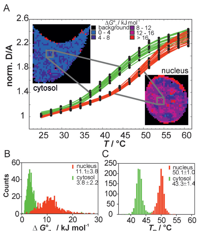
Figure 4. A) Single-pixel-based titration curves for cytosolic and nucleus regions of a single cell. Insets: False-colored images of the free energy of unfolding at 37°C, \Delta G^{\circ}_u , calculated for each pixel. B) \Delta G^{\circ}_u (37°C) and C) T_m single-pixel histograms of the cytosol and nucleus of the same cell as shown in (A).
