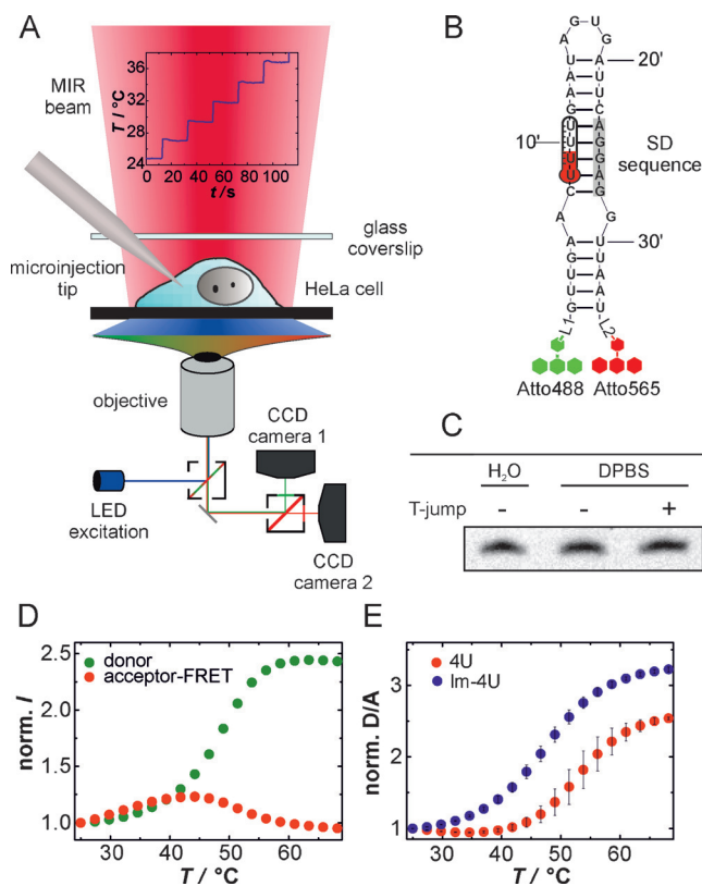
Figure 1. 4U RNA thermal unfolding studied by Fast Relaxation Imaging (FReI). A) Representation of the FReI setup. B) 4U structure labeled with FRET-capable dyes Atto488 and Atto565. SD = Shine-Dalgarno. For detailed structure of linker regions L1 and L2 see Figure S1. C) Gel electrophoresis and EtBr staining reveal the intactness of the hairpin after temperature stepping in DPBS buffer. D) Normalized donor- and acceptor-FRET fluorescence intensities for 4U RNA in DPBS buffer studied by FReI. E) Normalized D/A FRET signal as a function of temperature for 4U RNA and its low-melting variant G12A-C23U (Im-4U) in vitro. n=4 . Error bars represent mean \pm s.d.
